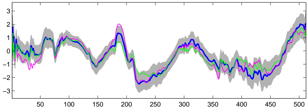
Estimated U_{19}(t) using R-WFMM: DE data, run 6
