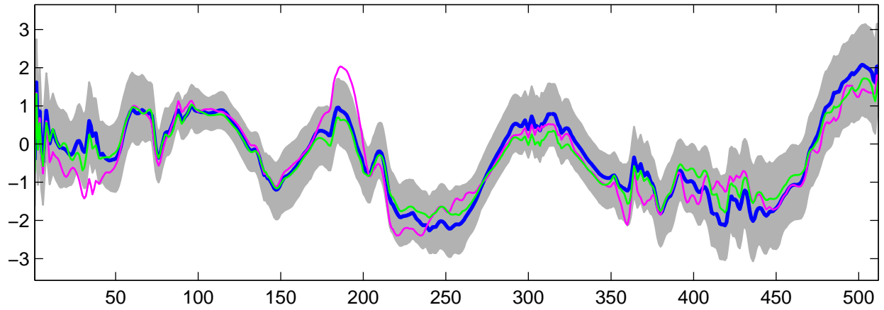
Estimated U_{19}(t) using G-WFMM: DE data, run 6
