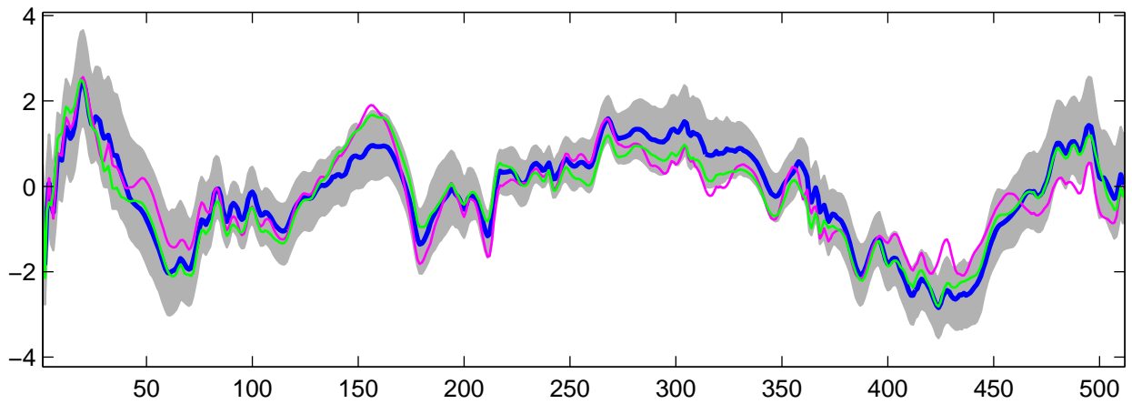
Estimated U_{19}(t) using R-WFMM: Normal data, run 6
