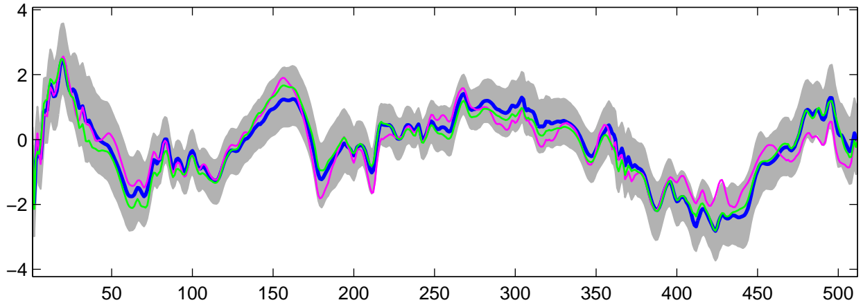
Estimated U_{19}(t) using G-WFMM: Normal data, run 6
