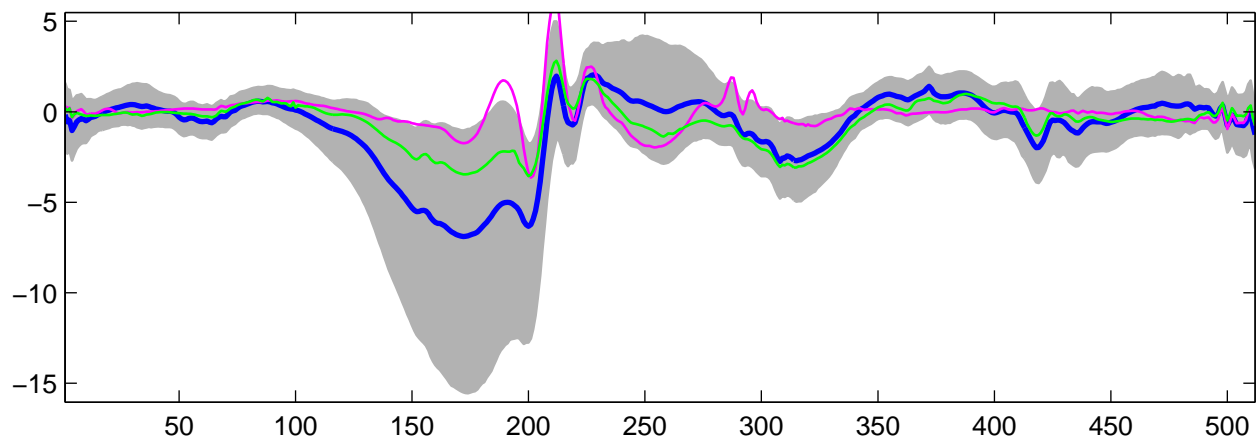
Estimated U_{19}(t) using G-WFMM: t_1 data, run 6
