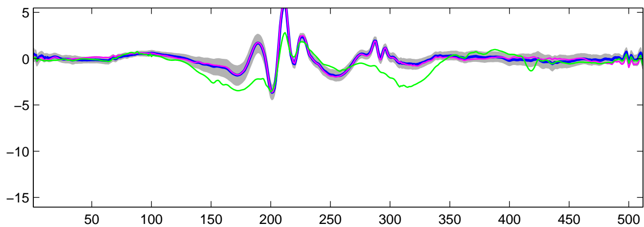
Estimated U_{19}(t) using R-WFMM: t_1 data, run 6
