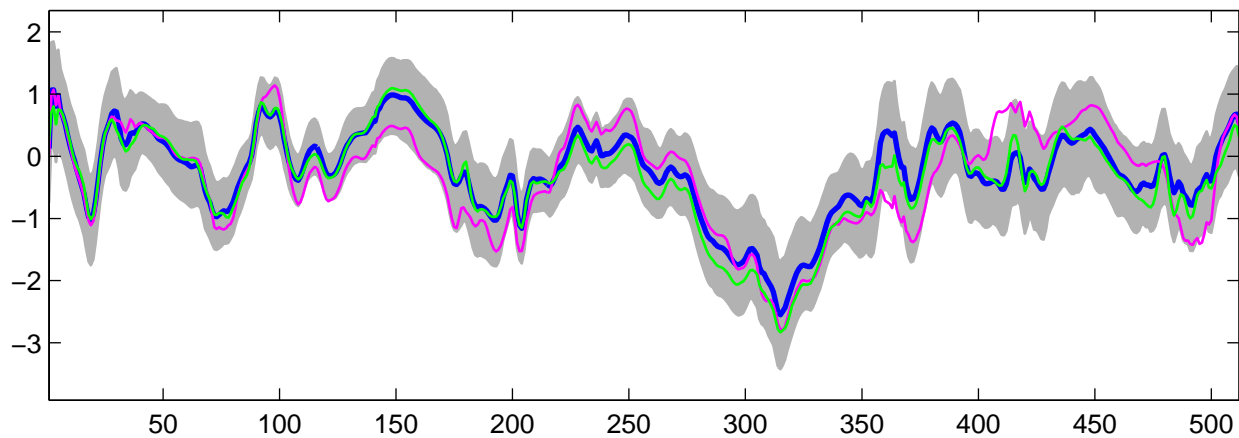
Estimated U_{19}(t) using G-WFMM: t_3 data, run 6
