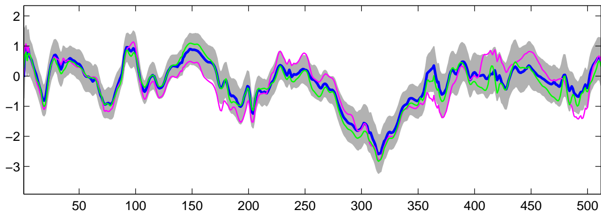
Estimated U_{19}(t) using R-WFMM: t_3 data, run 6
