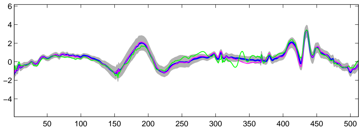
Estimated U_1(t) using R-WFMM: t_1 data, run 6
