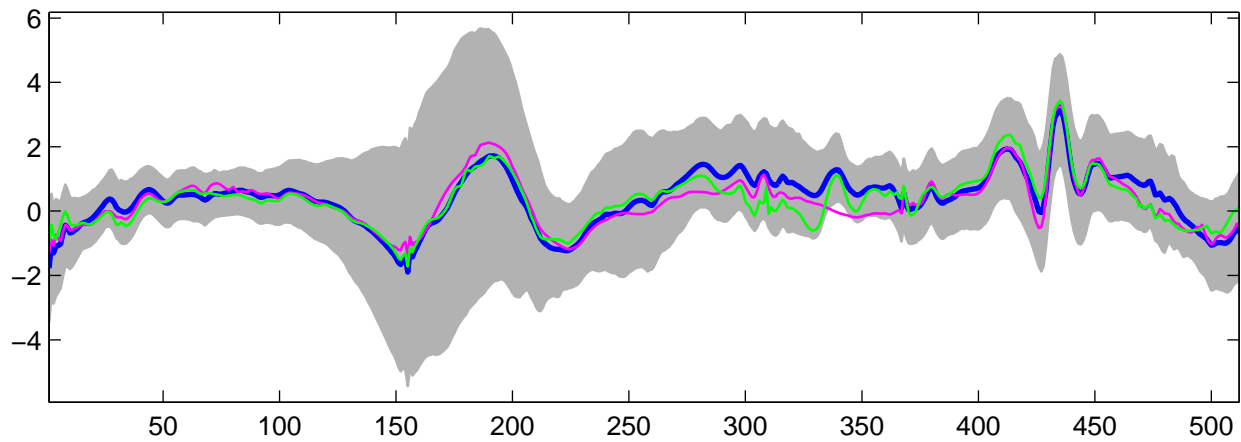
Estimated U_1(t) using G-WFMM: t_1 data, run 6
