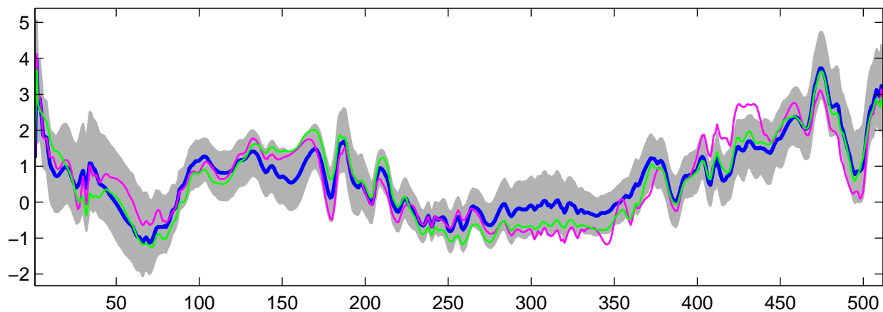
Estimated U_{20}(t) using R-WFMM: Normal data, run 6
