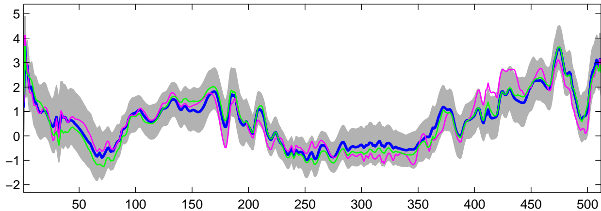
Estimated U_{20}(t) using G-WFMM: Normal data, run 6
