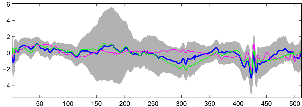
Estimated U_{20}(t) using G-WFMM: t_1 data, run 6
