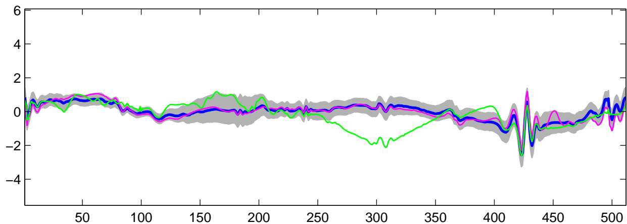
Estimated U_{20}(t) using R-WFMM: t_1 data, run 6
