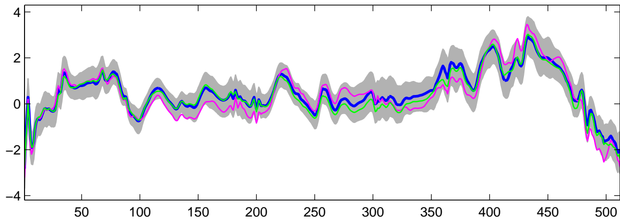
Estimated U_{20}(t) using G-WFMM: t_3 data, run 6
