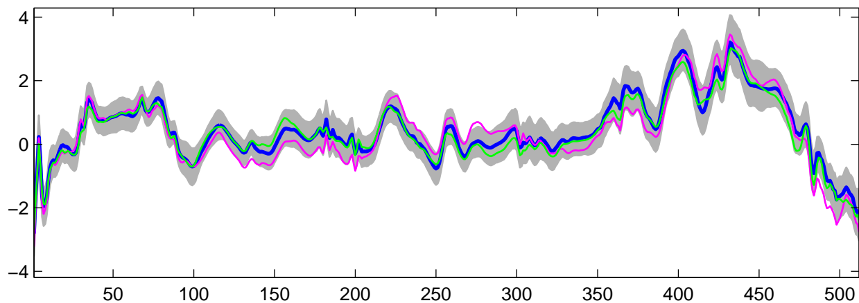
Estimated U_{20}(t) using R-WFMM: t_3 data, run 6
