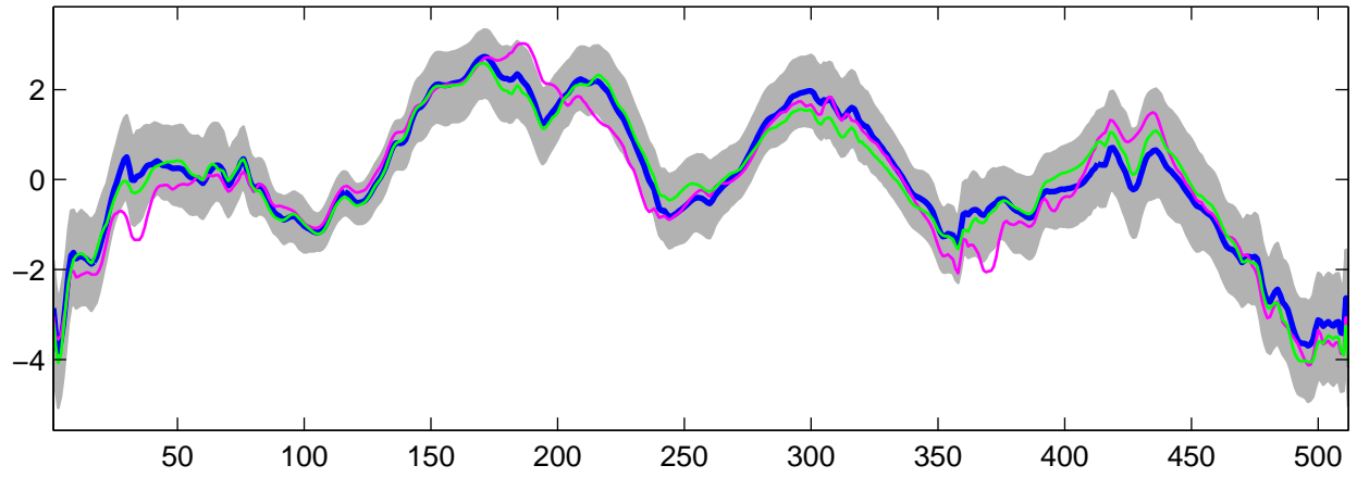
Estimated U_{21}(t) using G-WFMM: DE data, run 6
