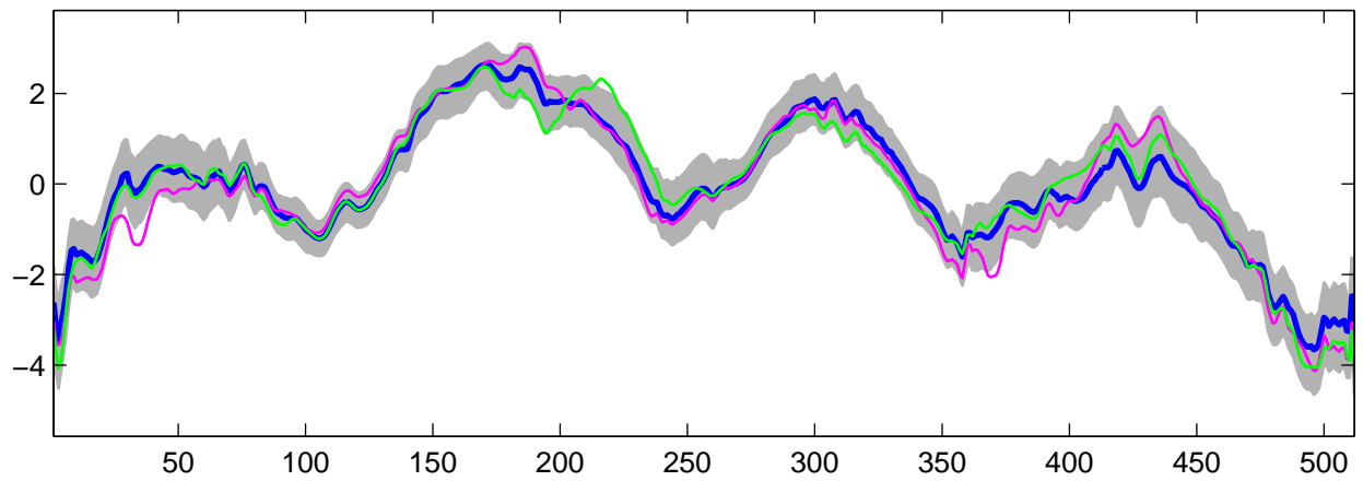
Estimated U_{21}(t) using R-WFMM: DE data, run 6
