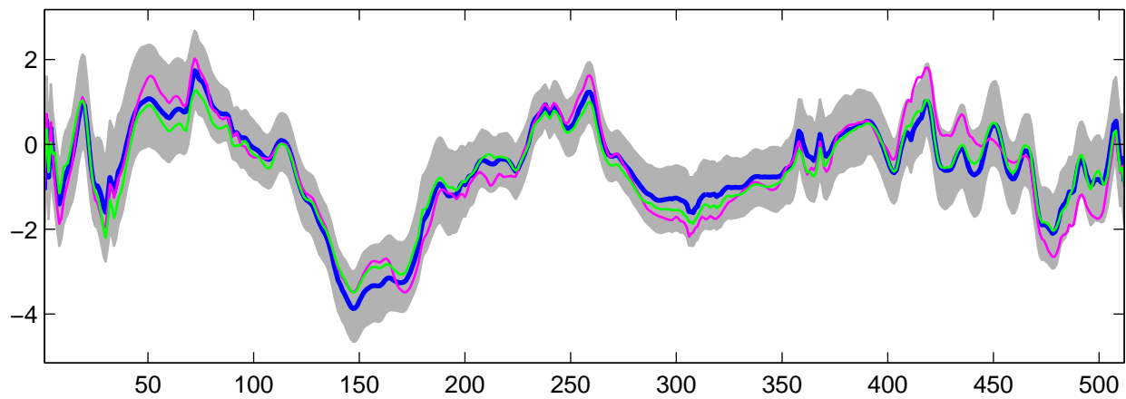
Estimated U_{21}(t) using G-WFMM: Normal data, run 6
