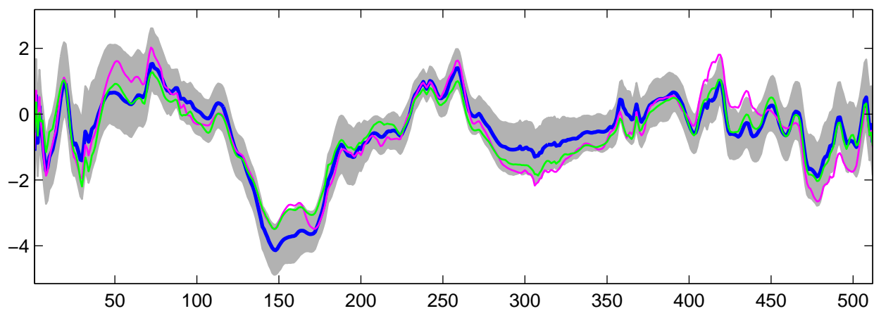
Estimated U_{21}(t) using R-WFMM: Normal data, run 6
