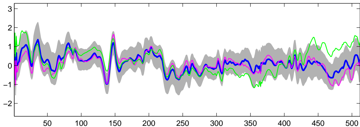
Estimated U_{21}(t) using R-WFMM: t_2 data, run 6
