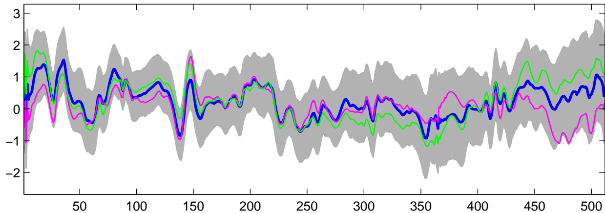
Estimated U_{21}(t) using G-WFMM: t_2 data, run 6
