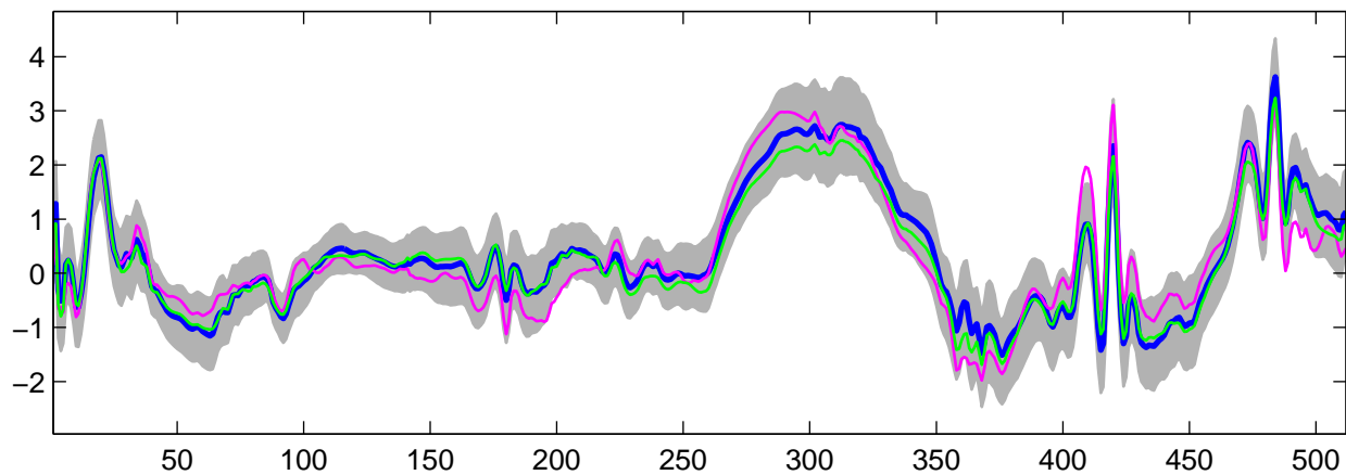
Estimated U_{21}(t) using G-WFMM: t_3 data, run 6
