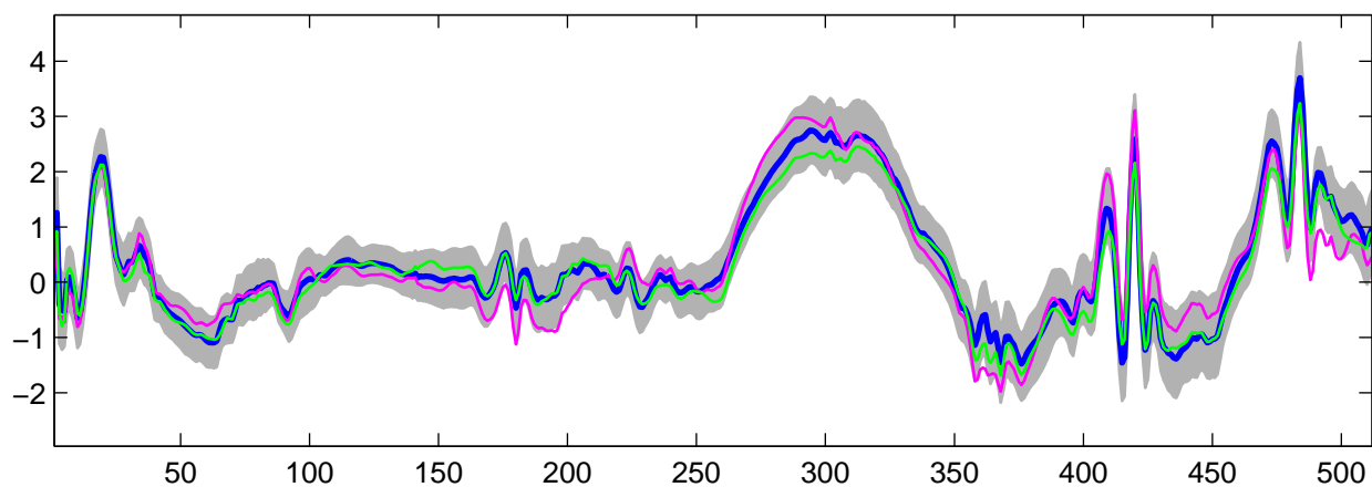
Estimated U_{21}(t) using R-WFMM: t_3 data, run 6
