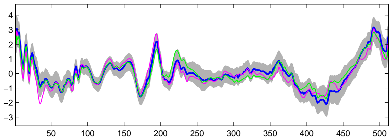
Estimated U_{22}(t) using R-WFMM: DE data, run 6
