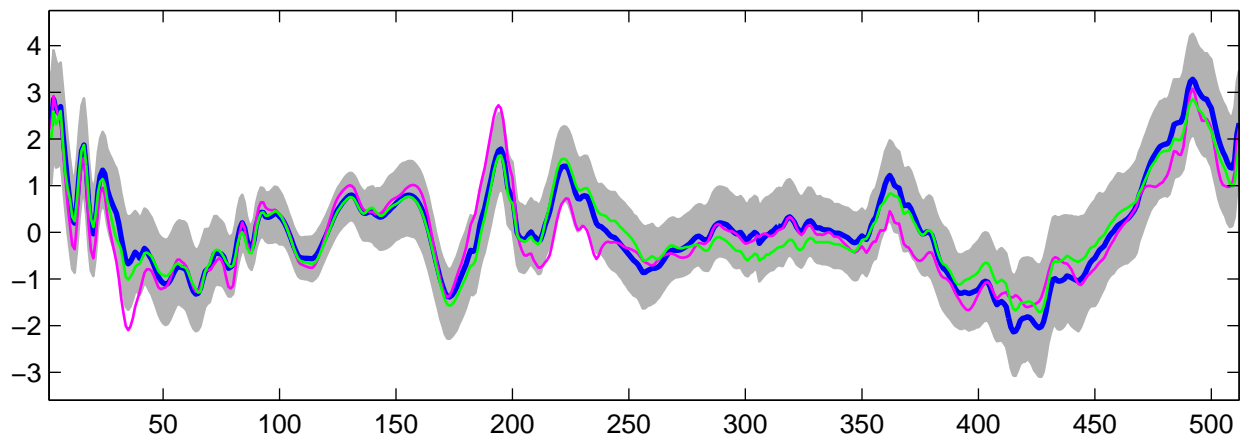
Estimated U_{22}(t) using G-WFMM: DE data, run 6
