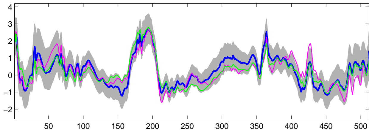
Estimated U_{22}(t) using R-WFMM: Normal data, run 6
