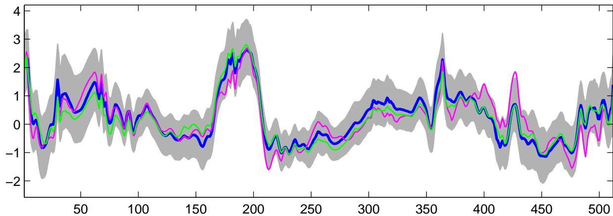
Estimated U_{22}(t) using G-WFMM: Normal data, run 6
