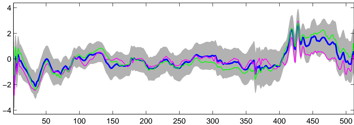
Estimated U_{22}(t) using G-WFMM: t_2 data, run 6
