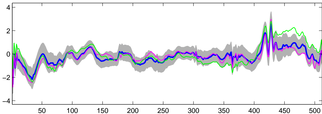
Estimated U_{22}(t) using R-WFMM: t_2 data, run 6
