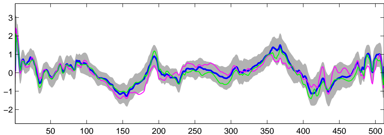
Estimated U_{22}(t) using R-WFMM: t_3 data, run 6
