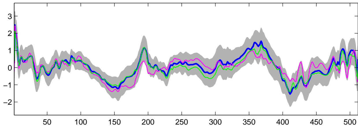
Estimated U_{22}(t) using G-WFMM: t_3 data, run 6
