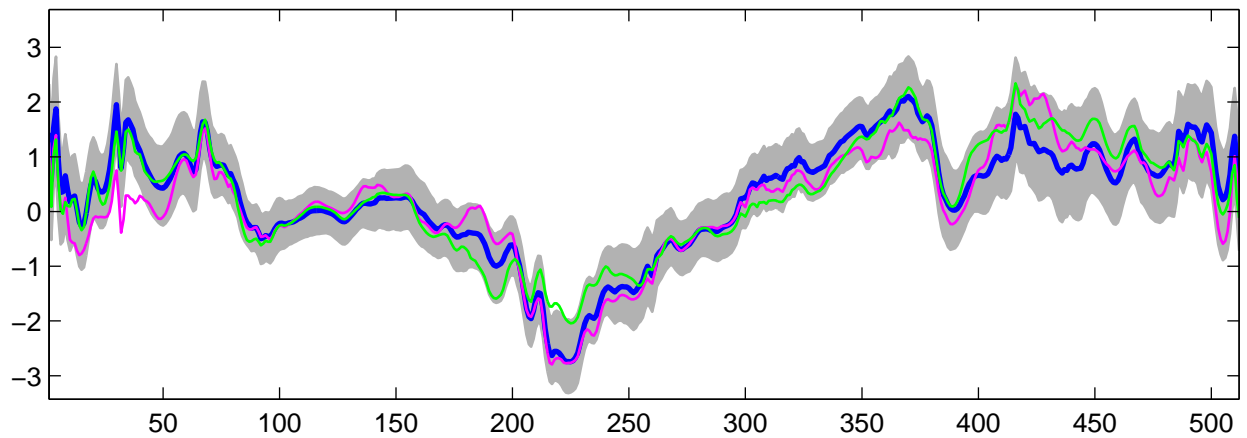
Estimated U_{23}(t) using R-WFMM: DE data, run 6
