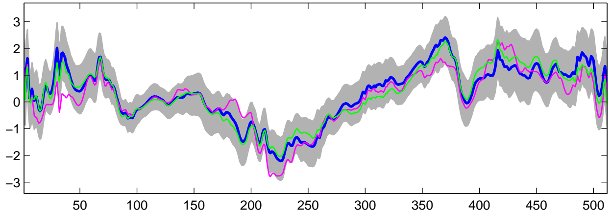
Estimated U_{23}(t) using G-WFMM: DE data, run 6
