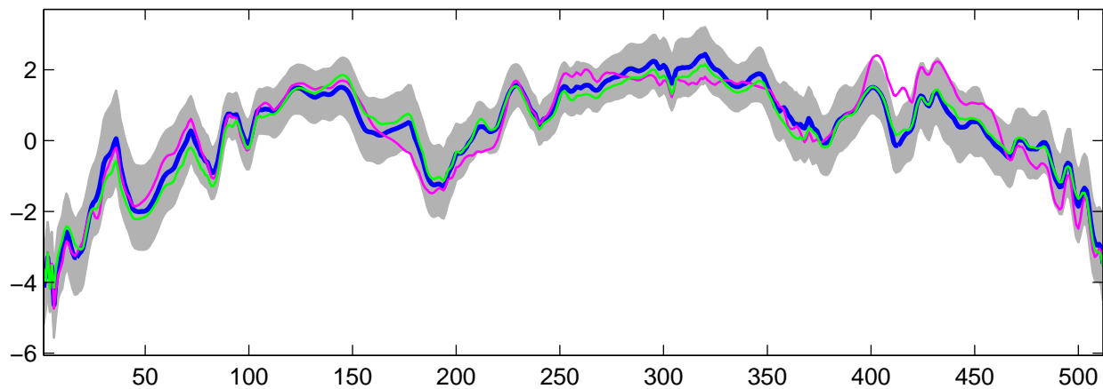
Estimated U_{23}(t) using G-WFMM: Normal data, run 6
