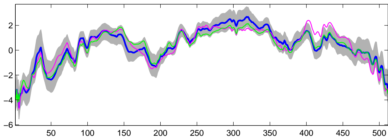
Estimated U_{23}(t) using R-WFMM: Normal data, run 6
