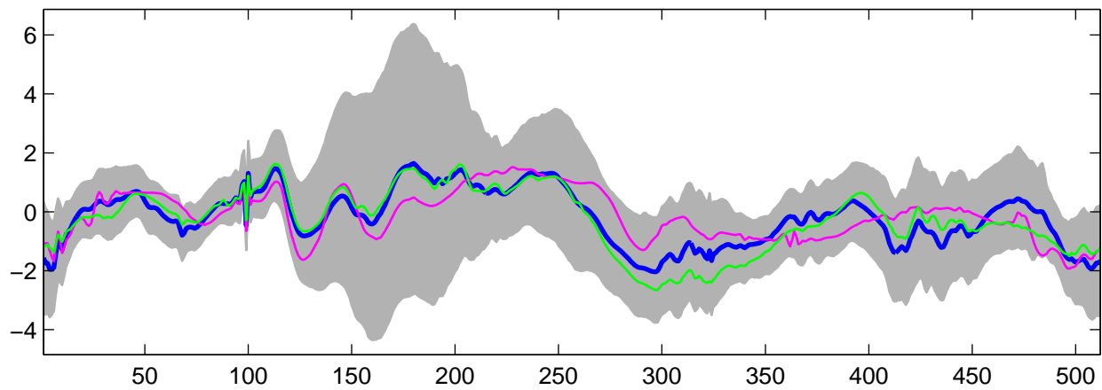
Estimated U_{23}(t) using G-WFMM: t_1 data, run 6
