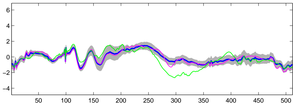
Estimated U_{23}(t) using R-WFMM: t_1 data, run 6
