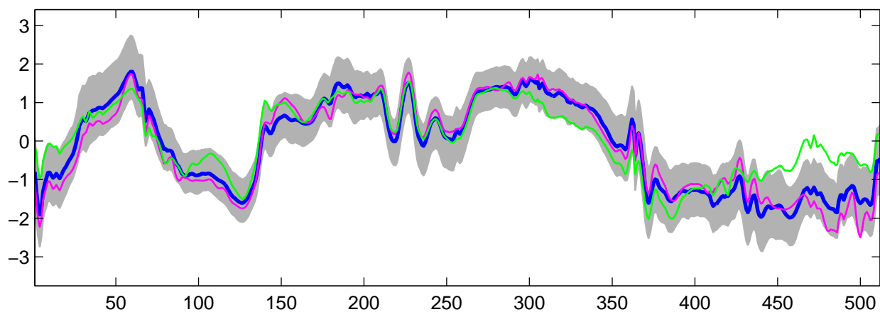
Estimated U_{23}(t) using R-WFMM: t_2 data, run 6
