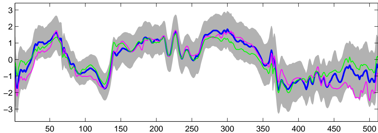
Estimated U_{23}(t) using G-WFMM: t_2 data, run 6
