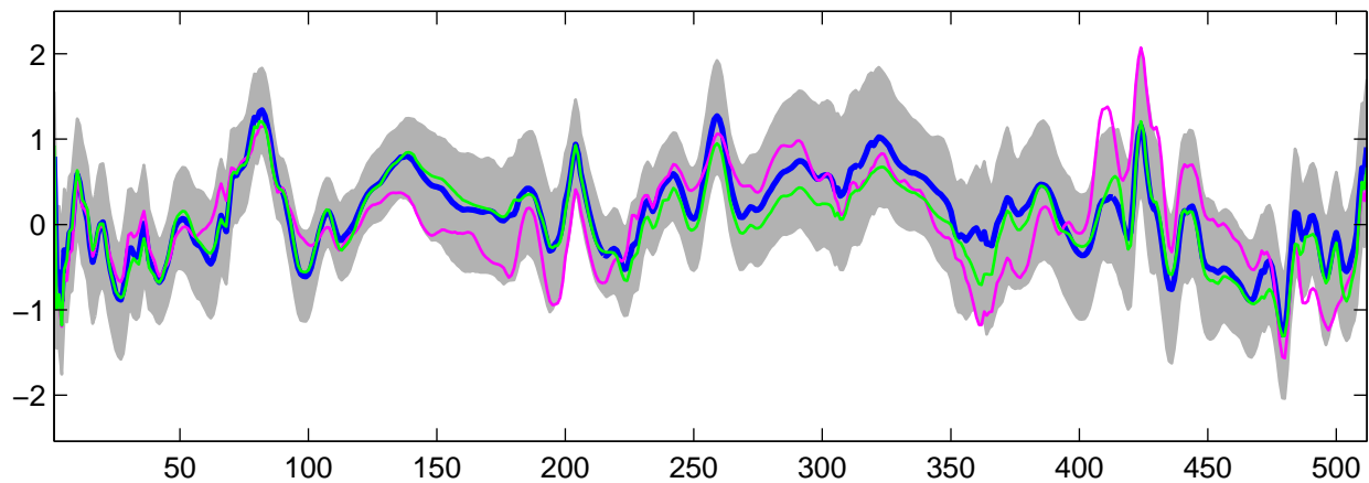
Estimated U_{23}(t) using G-WFMM: t_3 data, run 6
