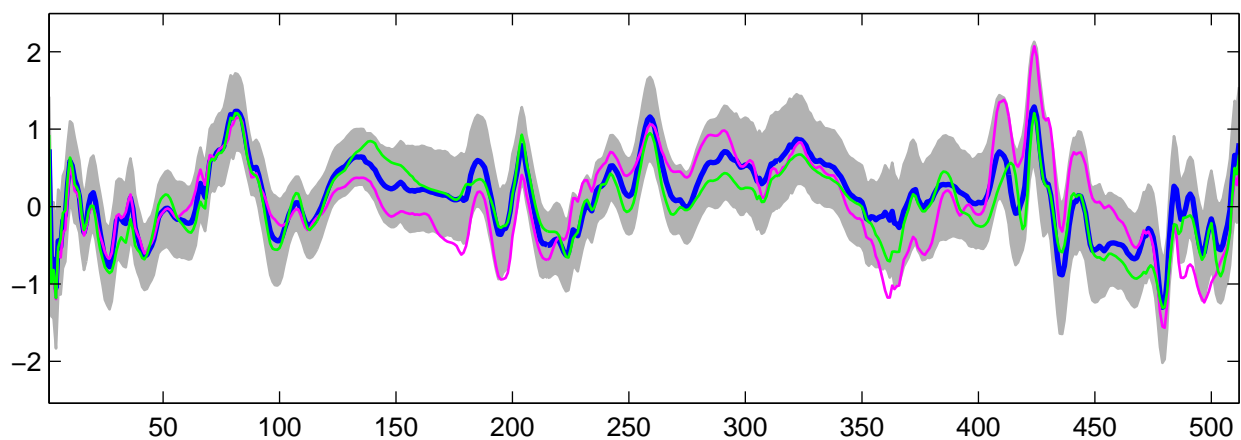
Estimated U_{23}(t) using R-WFMM: t_3 data, run 6
