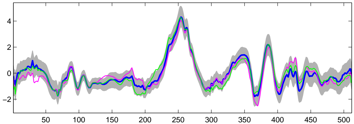
Estimated U_{24}(t) using R-WFMM: DE data, run 6
