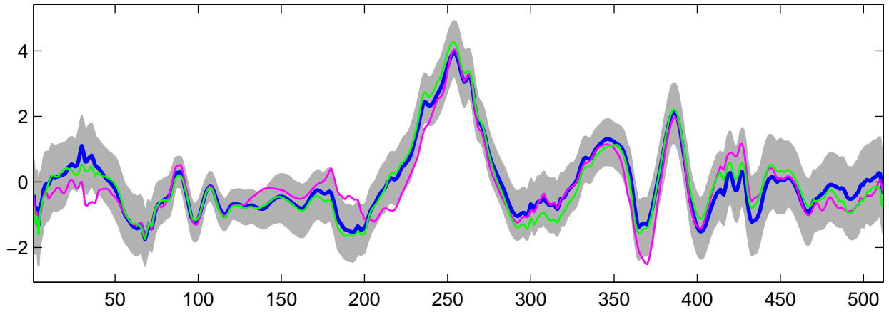
Estimated U_{24}(t) using G-WFMM: DE data, run 6
