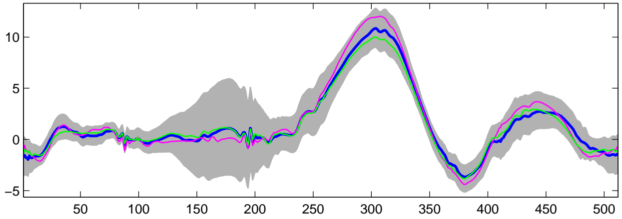
Estimated U_{24}(t) using G-WFMM: t_1 data, run 6
