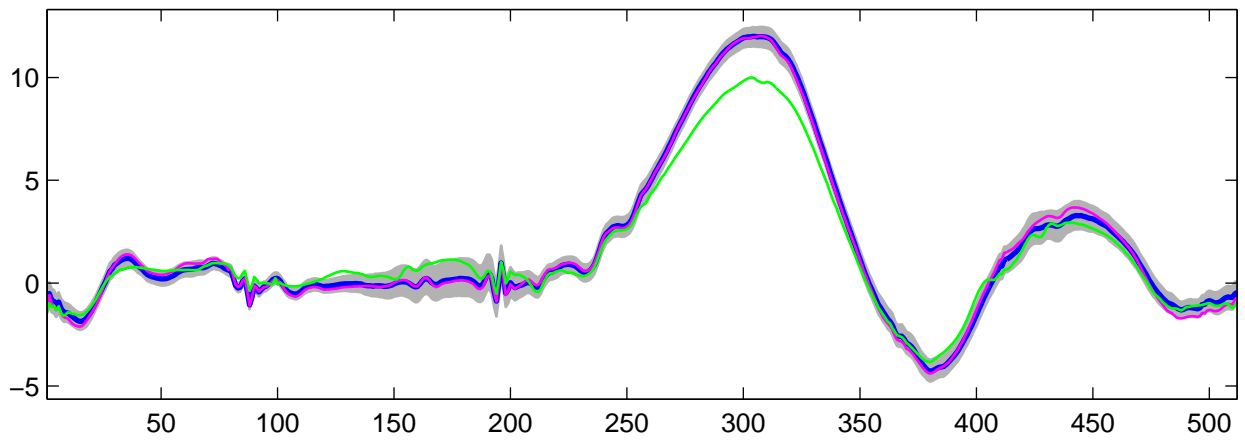
Estimated U_{24}(t) using R-WFMM: t_1 data, run 6
