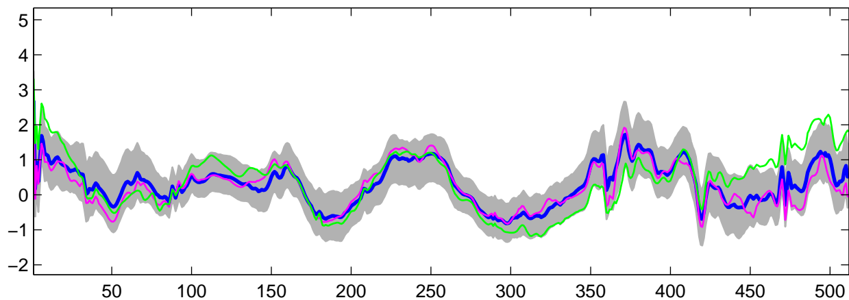
Estimated U_{24}(t) using R-WFMM: t_2 data, run 6
