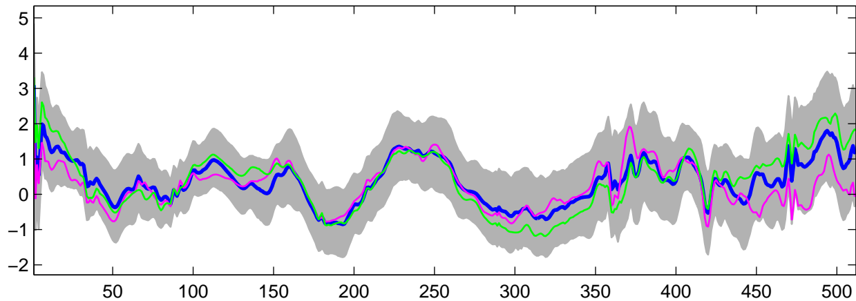
Estimated U_{24}(t) using G-WFMM: t_2 data, run 6
