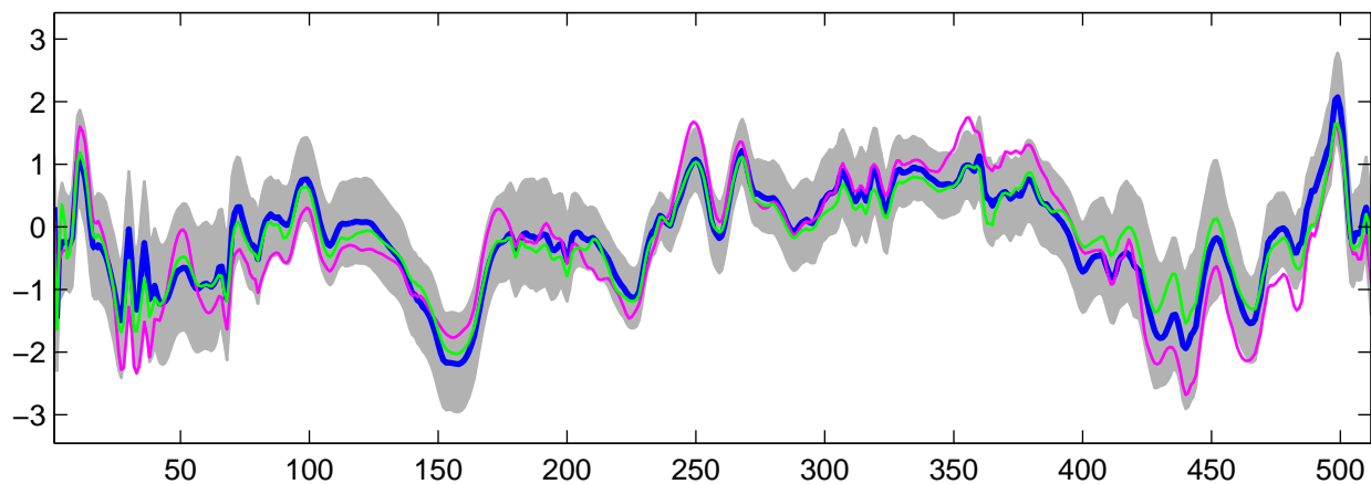
Estimated U_{25}(t) using R-WFMM: Normal data, run 6
