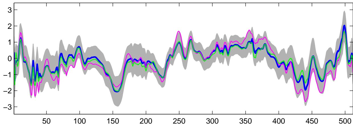
Estimated U_{25}(t) using G-WFMM: Normal data, run 6
