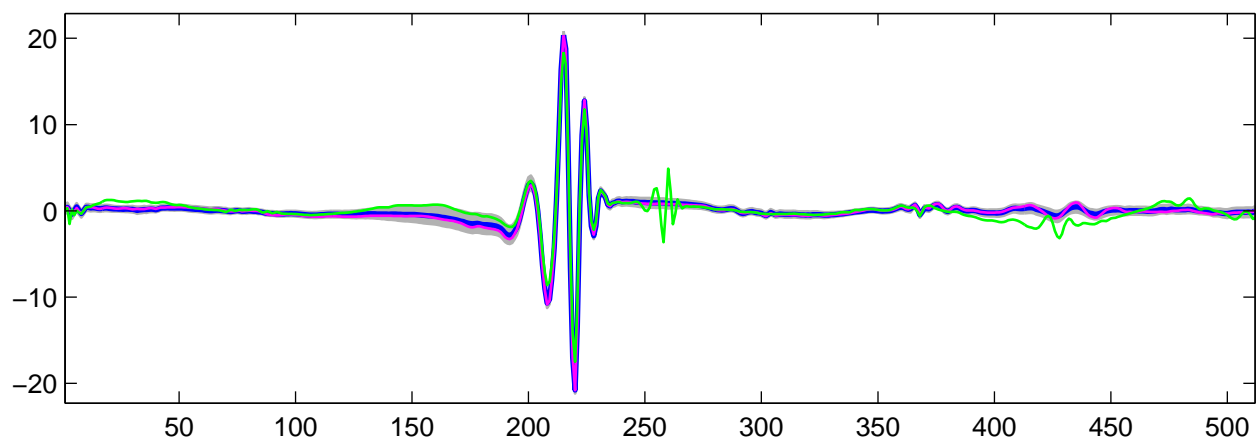
Estimated U_{25}(t) using R-WFMM: t_1 data, run 6
