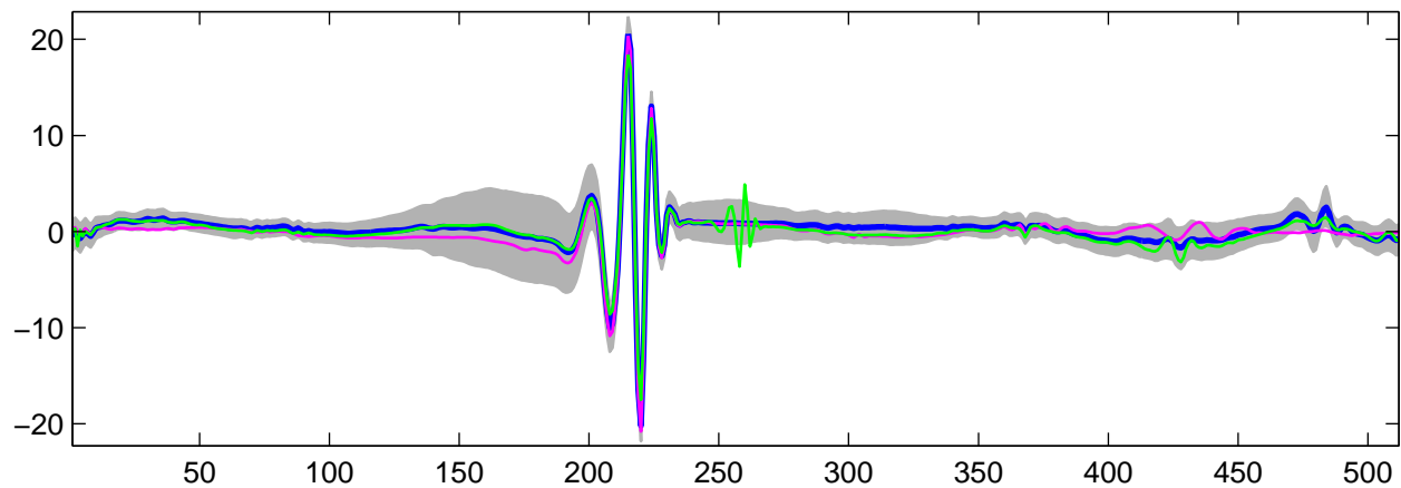
Estimated U_{25}(t) using G-WFMM: t_1 data, run 6
