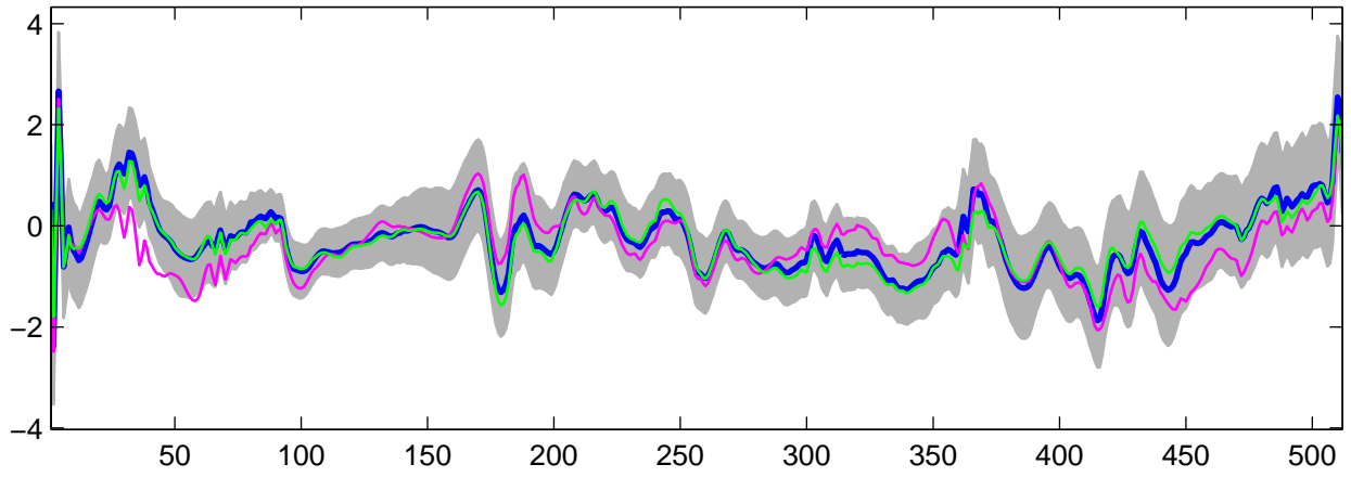
Estimated U_{26}(t) using G-WFMM: DE data, run 6
