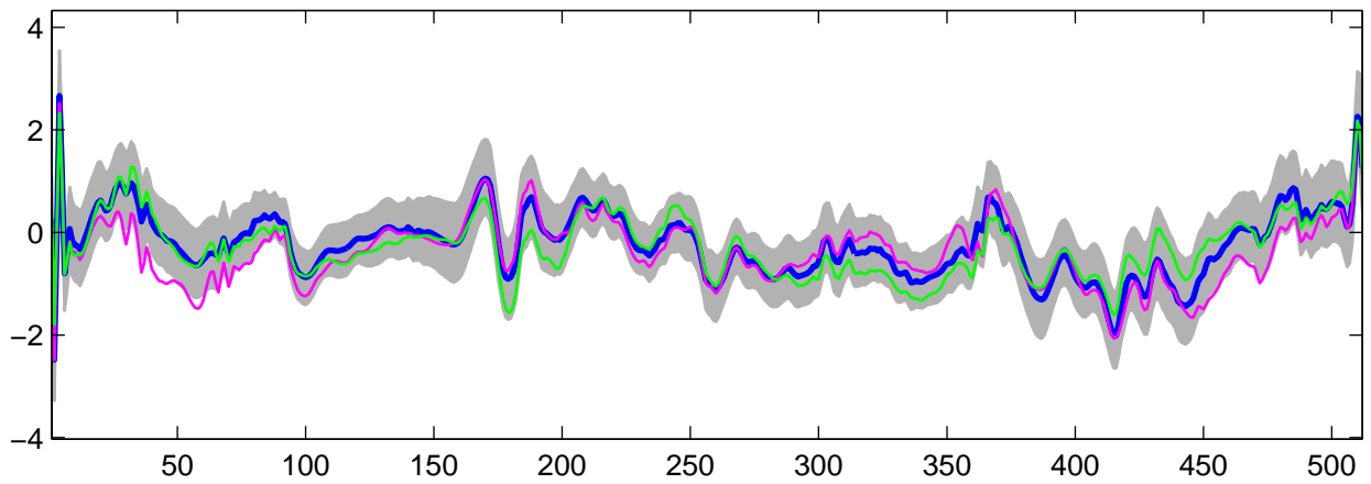
Estimated U_{26}(t) using R-WFMM: DE data, run 6
