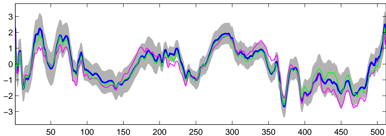
Estimated U_{26}(t) using R-WFMM: Normal data, run 6
