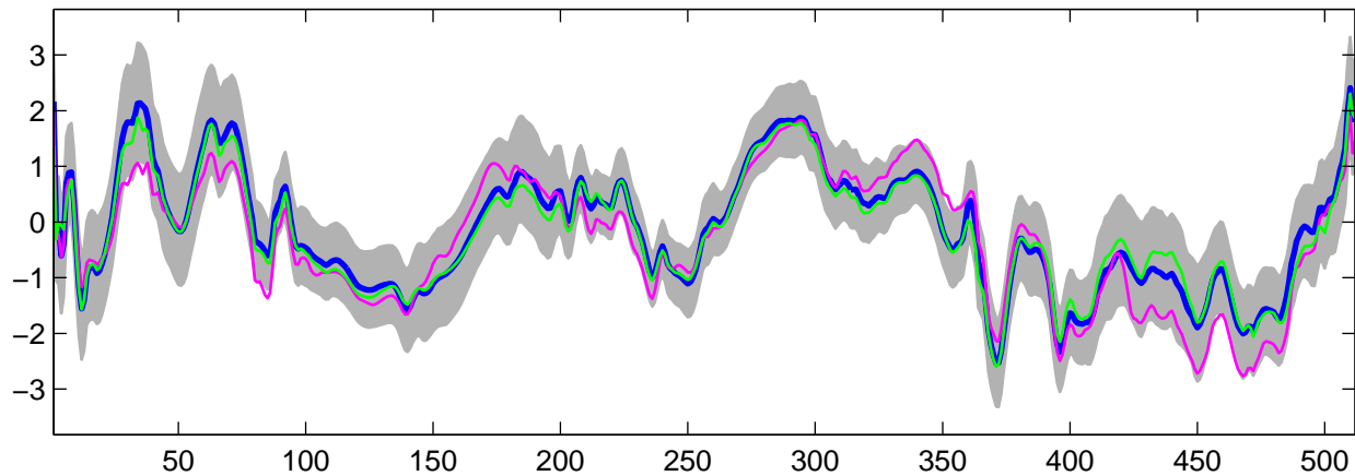
Estimated U_{26}(t) using G-WFMM: Normal data, run 6
