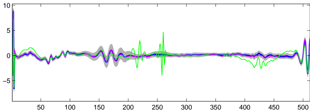
Estimated U_{26}(t) using R-WFMM: t_1 data, run 6
