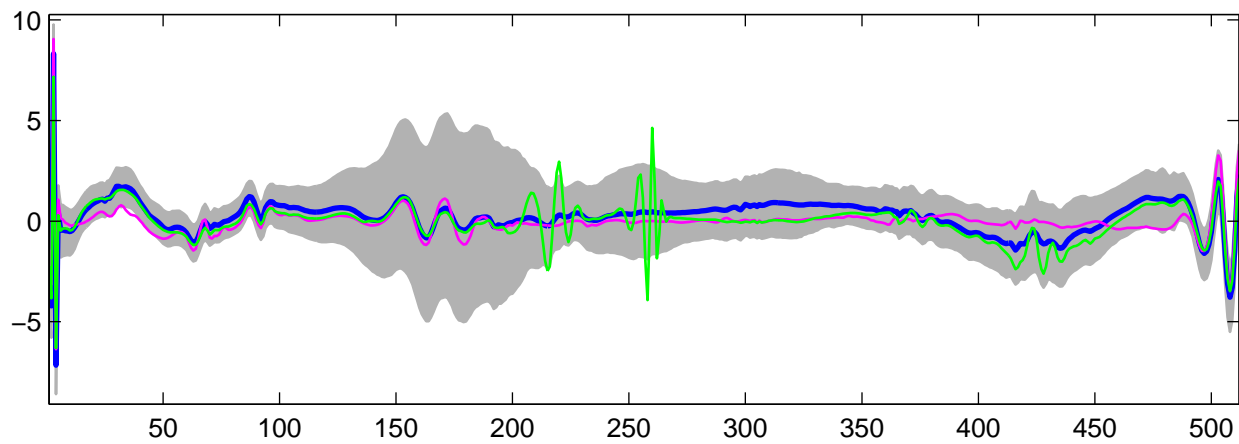
Estimated U_{26}(t) using G-WFMM: t_1 data, run 6
