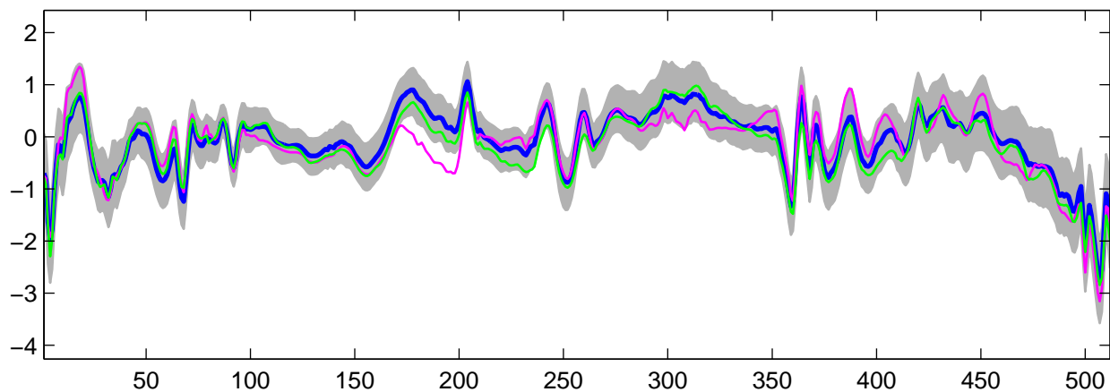
Estimated U_{26}(t) using R-WFMM: t_3 data, run 6
