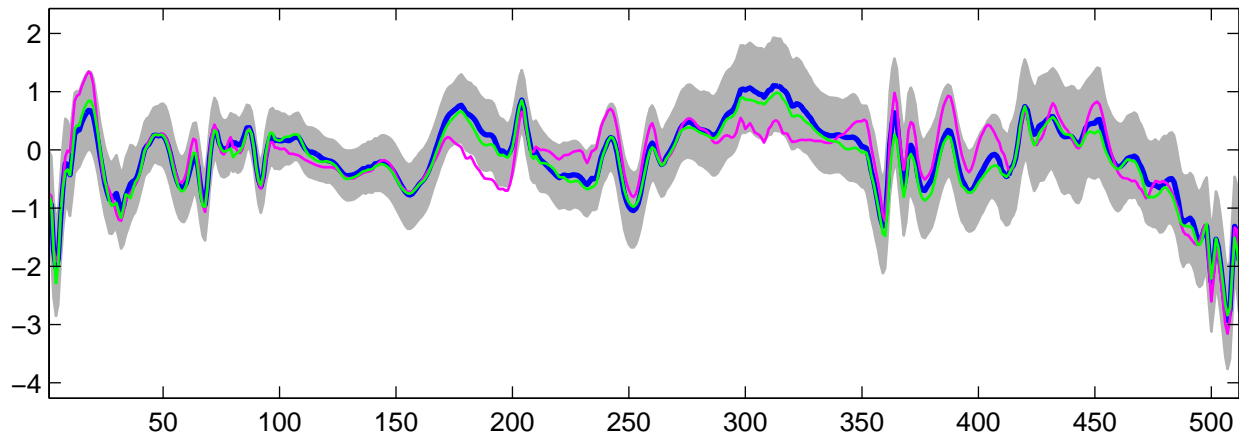
Estimated U_{26}(t) using G-WFMM: t_3 data, run 6
