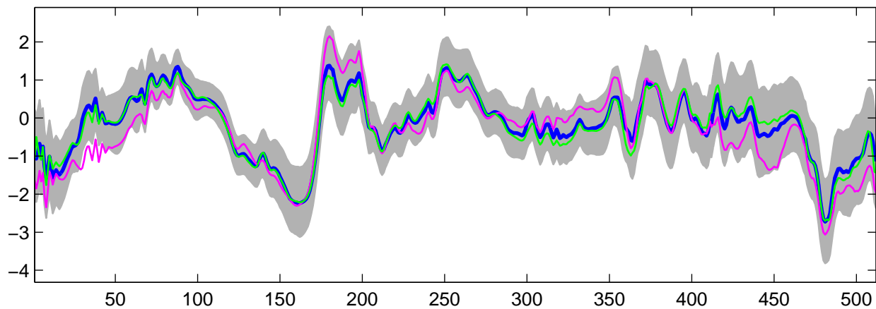
Estimated U_{27}(t) using G-WFMM: DE data, run 6
