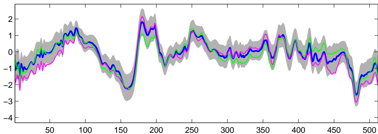
Estimated U_{27}(t) using R-WFMM: DE data, run 6
