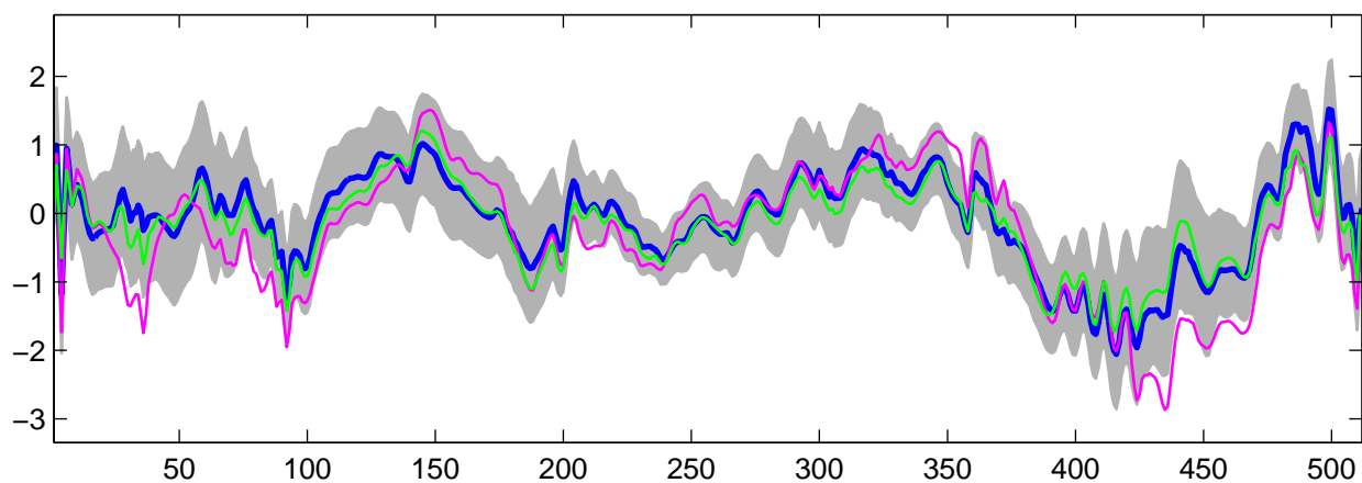
Estimated U_{27}(t) using R-WFMM: Normal data, run 6
