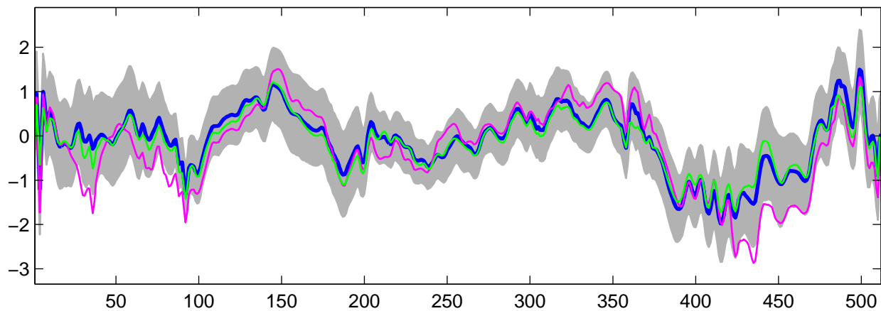
Estimated U_{27}(t) using G-WFMM: Normal data, run 6
