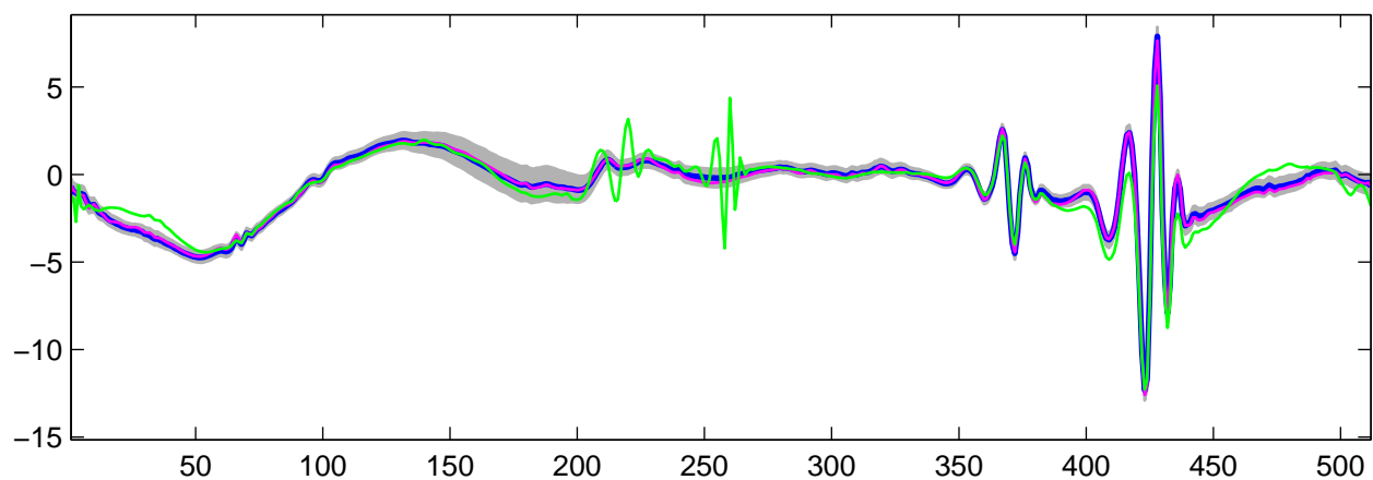
Estimated U_{27}(t) using R-WFMM: t_1 data, run 6
