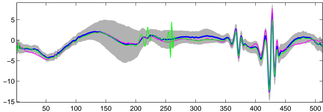
Estimated U_{27}(t) using G-WFMM: t_1 data, run 6
