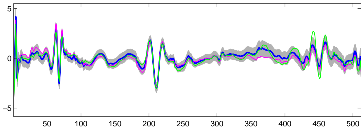
Estimated U_{27}(t) using R-WFMM: t_2 data, run 6
