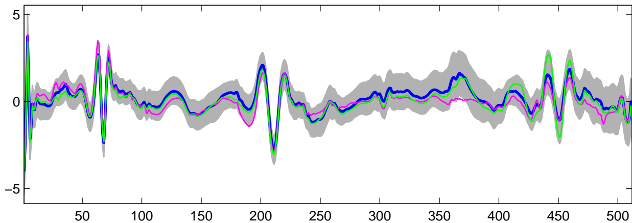
Estimated U_{27}(t) using G-WFMM: t_2 data, run 6
