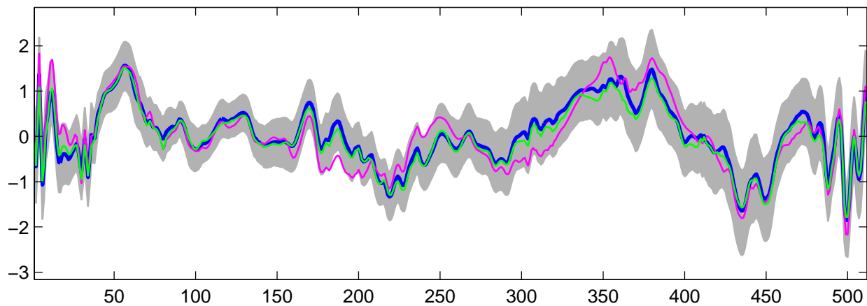
Estimated U_{27}(t) using G-WFMM: t_3 data, run 6
