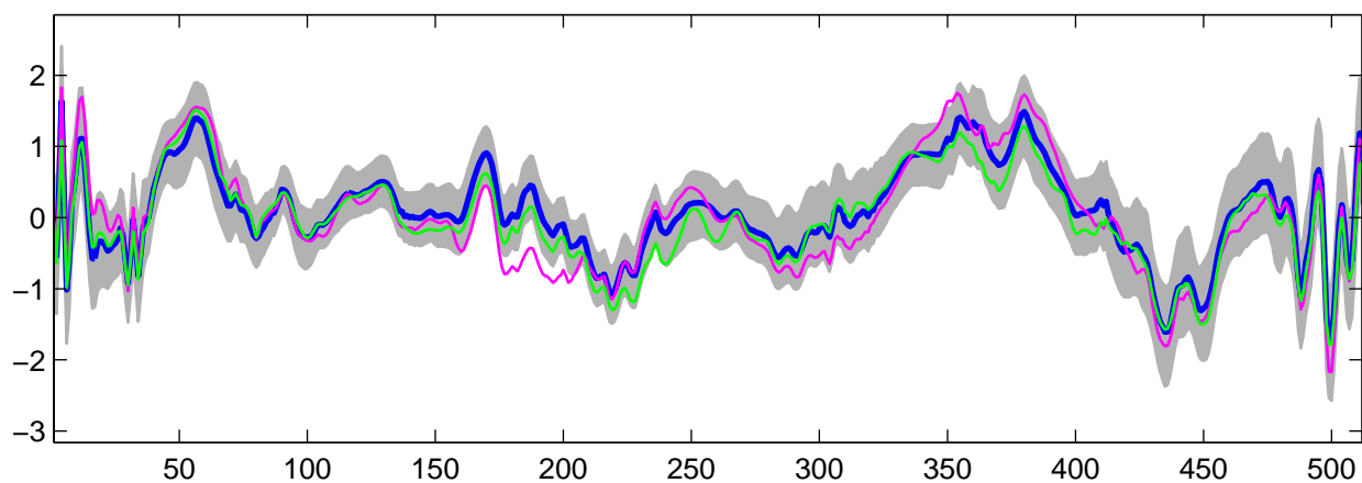
Estimated U_{27}(t) using R-WFMM: t_3 data, run 6
