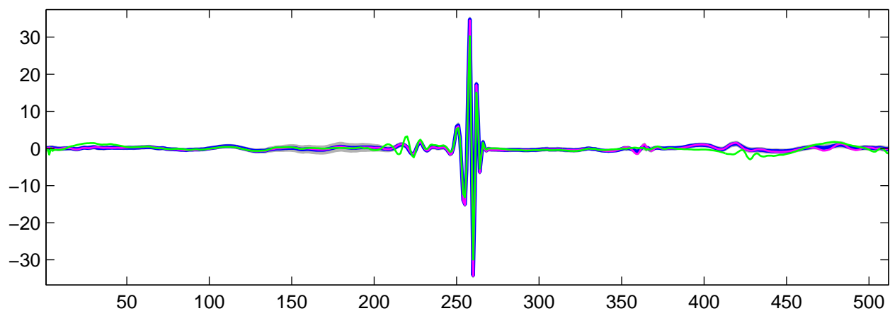
Estimated U_{28}(t) using R-WFMM: t_1 data, run 6
