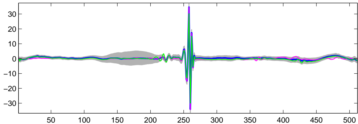
Estimated U_{28}(t) using G-WFMM: t_1 data, run 6
