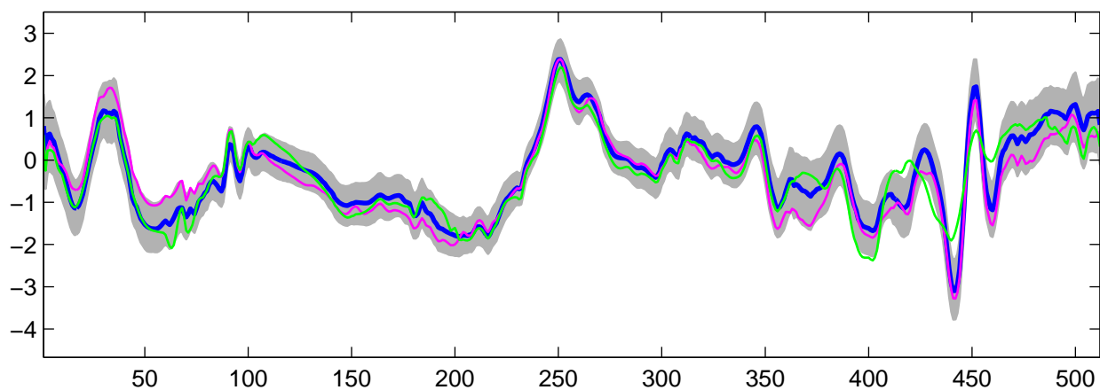
Estimated U_{28}(t) using R-WFMM: t_2 data, run 6
