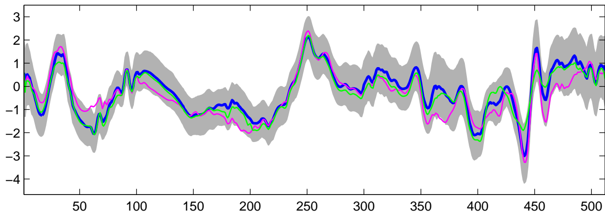
Estimated U_{28}(t) using G-WFMM: t_2 data, run 6
