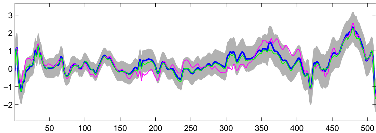
Estimated U_{28}(t) using G-WFMM: t_3 data, run 6
