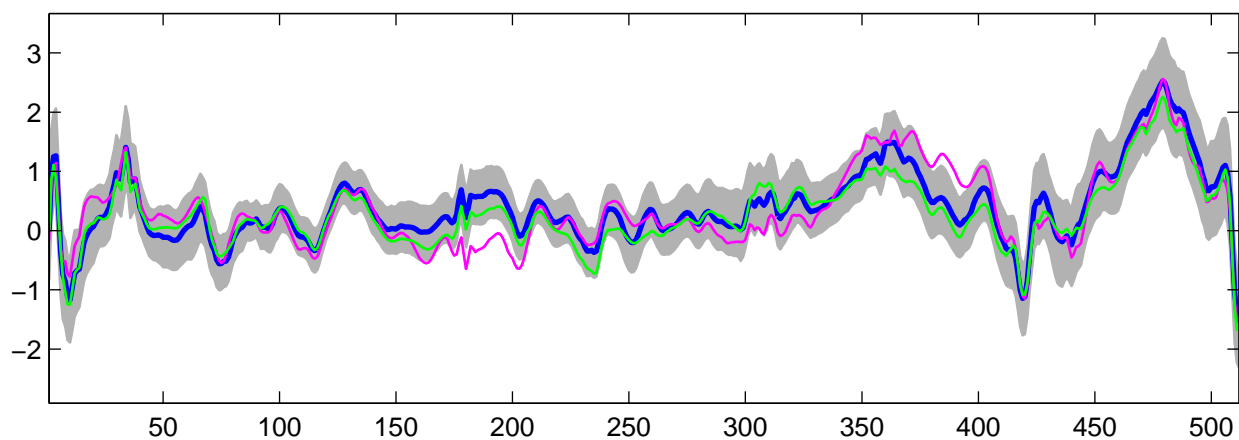
Estimated U_{28}(t) using R-WFMM: t_3 data, run 6
