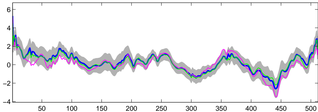
Estimated U_{29}(t) using G-WFMM: Normal data, run 6
