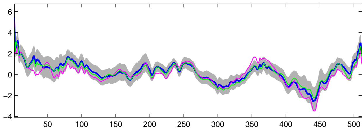
Estimated U_{29}(t) using R-WFMM: Normal data, run 6
