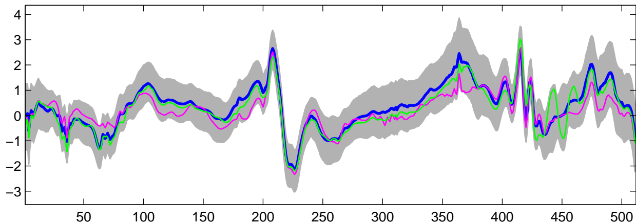
Estimated U_{29}(t) using G-WFMM: t_2 data, run 6
