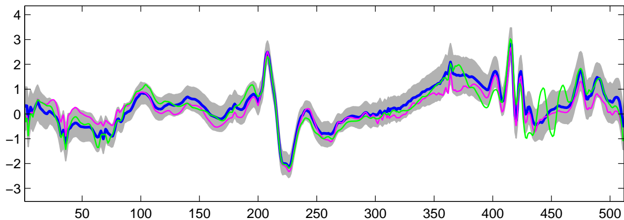
Estimated U_{29}(t) using R-WFMM: t_2 data, run 6
