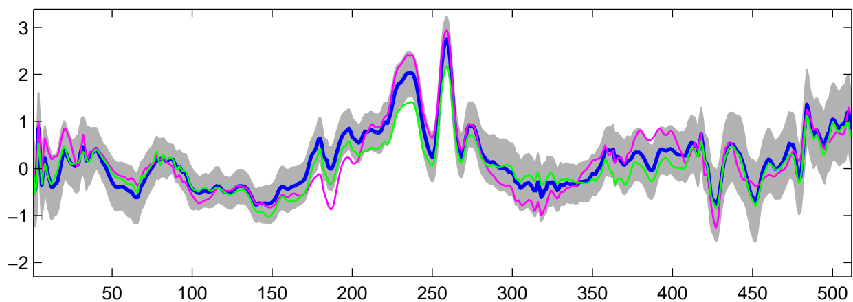
Estimated U_{29}(t) using R-WFMM: t_3 data, run 6
