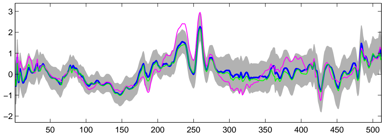
Estimated U_{29}(t) using G-WFMM: t_3 data, run 6
