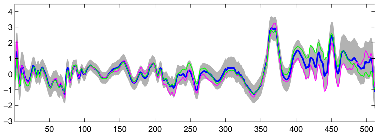
Estimated U_2(t) using R-WFMM: DE data, run 6
