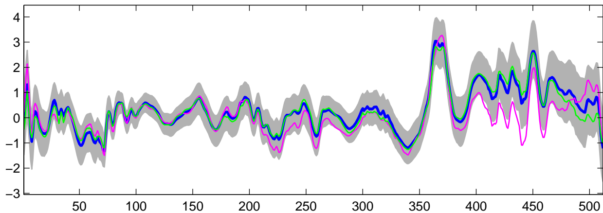
Estimated U_2(t) using G-WFMM: DE data, run 6
