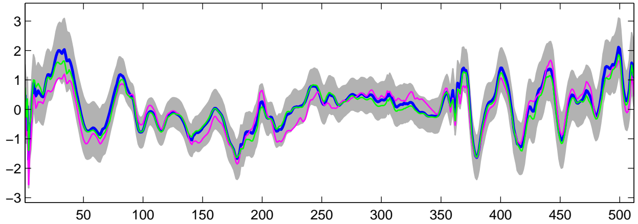
Estimated U_2(t) using G-WFMM: Normal data, run 6
