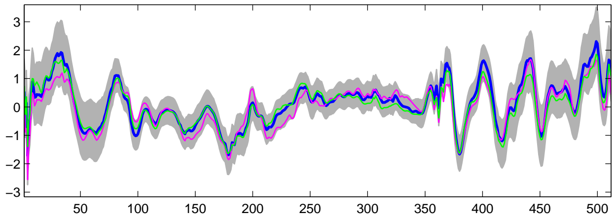
Estimated U_2(t) using R-WFMM: Normal data, run 6
