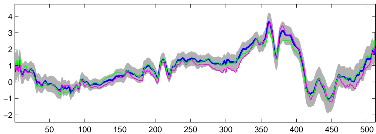
Estimated U_2(t) using R-WFMM: t_3 data, run 6
