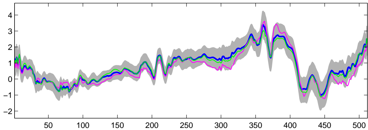
Estimated U_2(t) using G-WFMM: t_3 data, run 6
