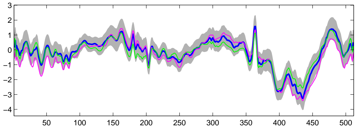
Estimated U_{30}(t) using R-WFMM: DE data, run 6
