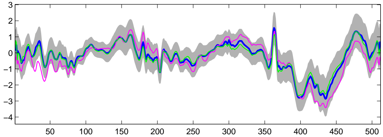
Estimated U_{30}(t) using G-WFMM: DE data, run 6
