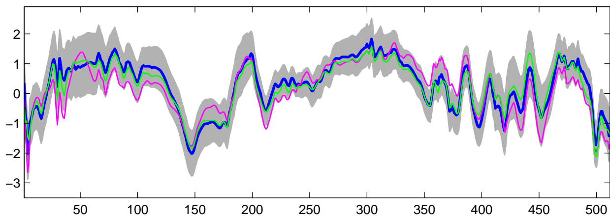
Estimated U_{30}(t) using R-WFMM: Normal data, run 6
