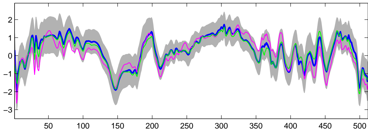
Estimated U_{30}(t) using G-WFMM: Normal data, run 6
