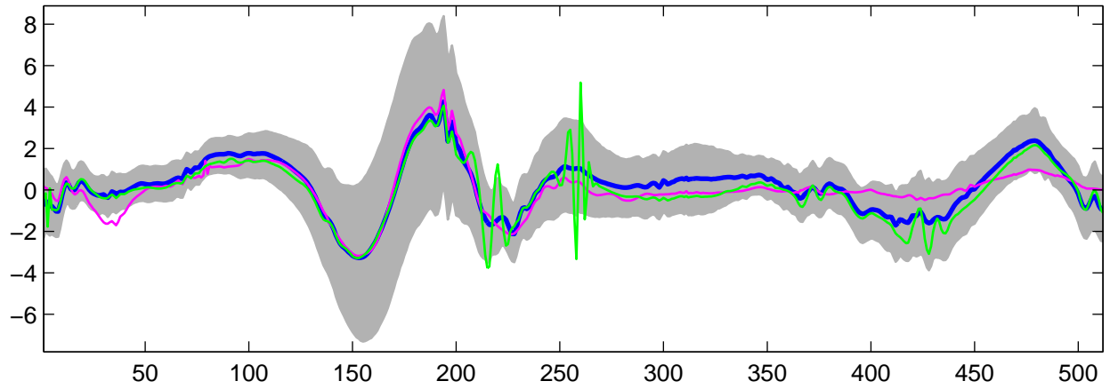
Estimated U_{30}(t) using G-WFMM: t_1 data, run 6
