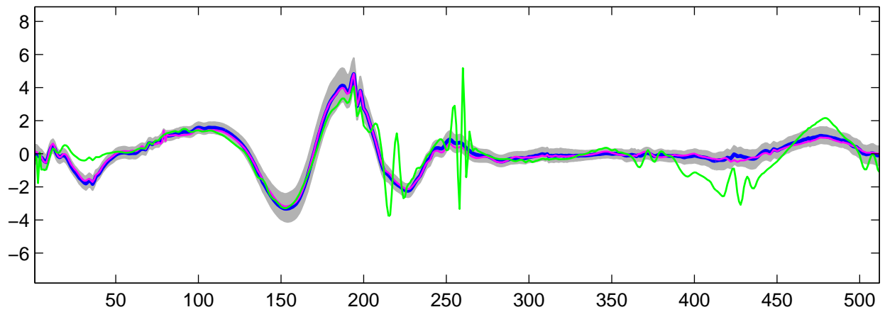
Estimated U_{30}(t) using R-WFMM: t_1 data, run 6
