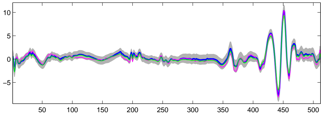
Estimated U_{30}(t) using G-WFMM: t_2 data, run 6
