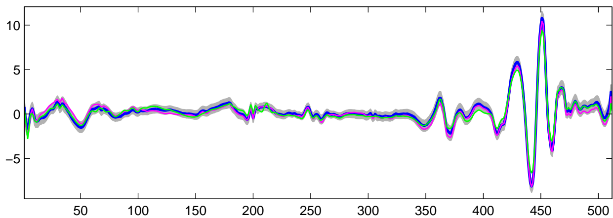
Estimated U_{30}(t) using R-WFMM: t_2 data, run 6
