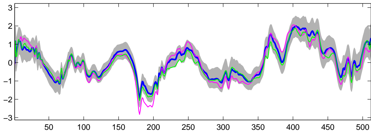
Estimated U_{30}(t) using R-WFMM: t_3 data, run 6
