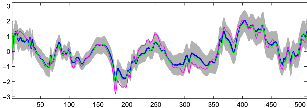
Estimated U_{30}(t) using G-WFMM: t_3 data, run 6
