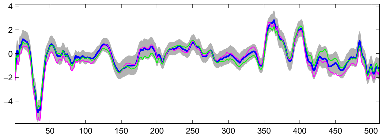
Estimated U_{31}(t) using R-WFMM: DE data, run 6
